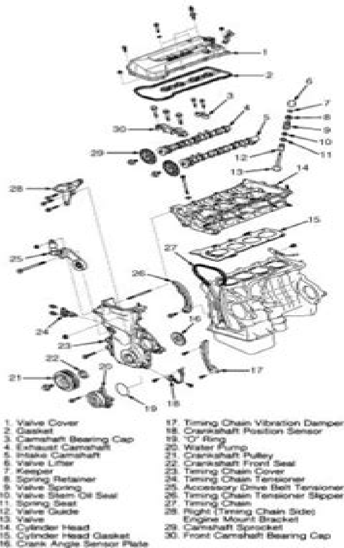
Fig. 6: Exploded View Of Cylinder Head & Timing Chain Components Courtesy of TOYOTA MOTOR SALES, U.S.A., INC.
