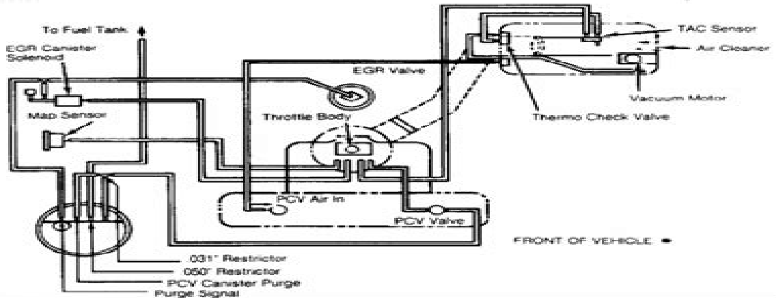
Fig. 11 2.5L 4-Cylinder Courtesy of Chrysler Motors.
