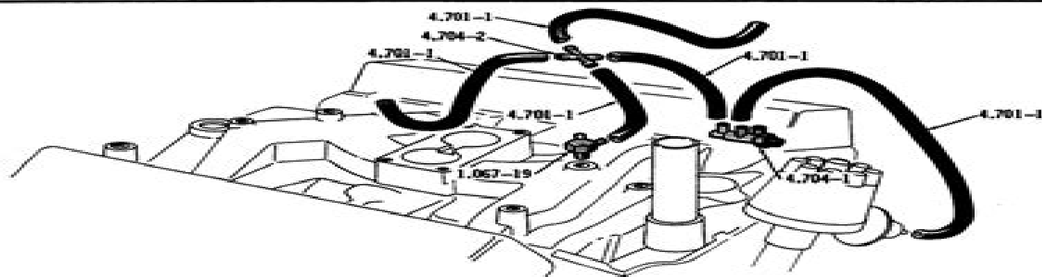
VACUUM ADVANCE MODULATION SYSTEM . . . 10-25-45 (V8-WHDC-CALIF), 1974 80 (V8-CALIF), 1975 80 (V8-E/CALIF)
