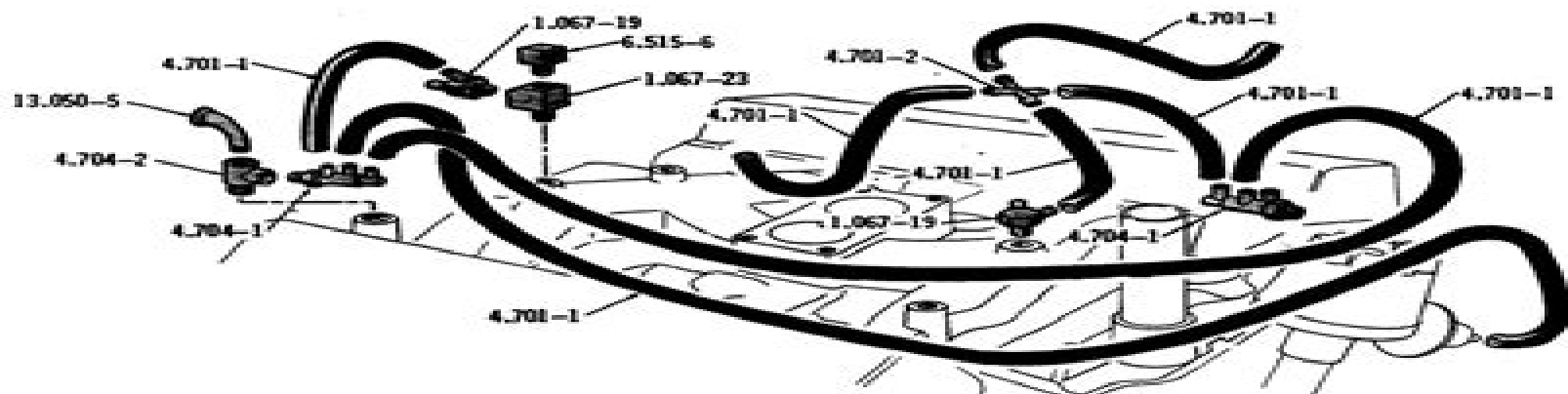
VACUUM ADVANCE MODULATION SYSTEM . . . 10-25-45 (V8-LHDC-CALIF)
