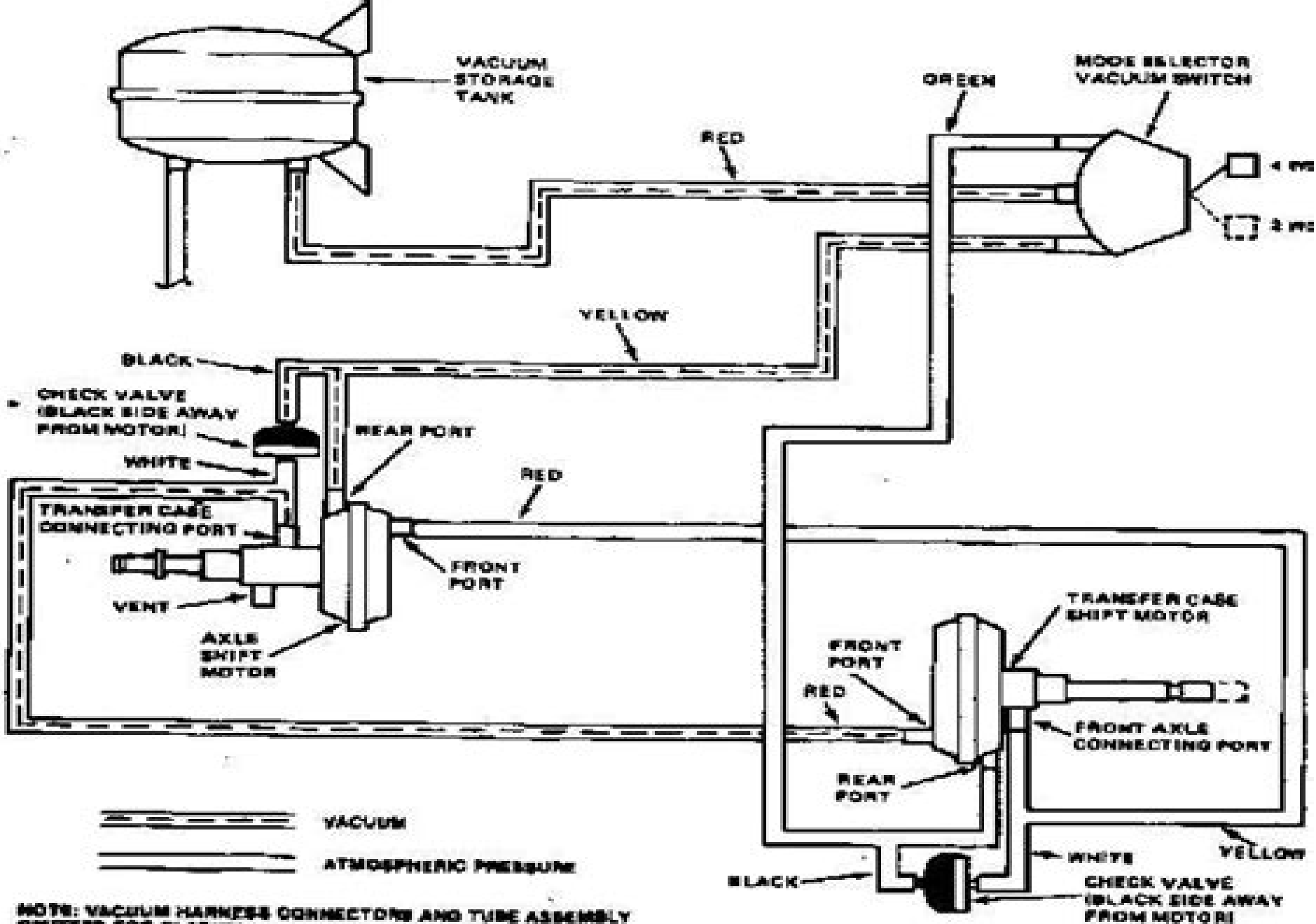
Fig. 14 Front Axle Vacuum Circuit. 4WD Mode
