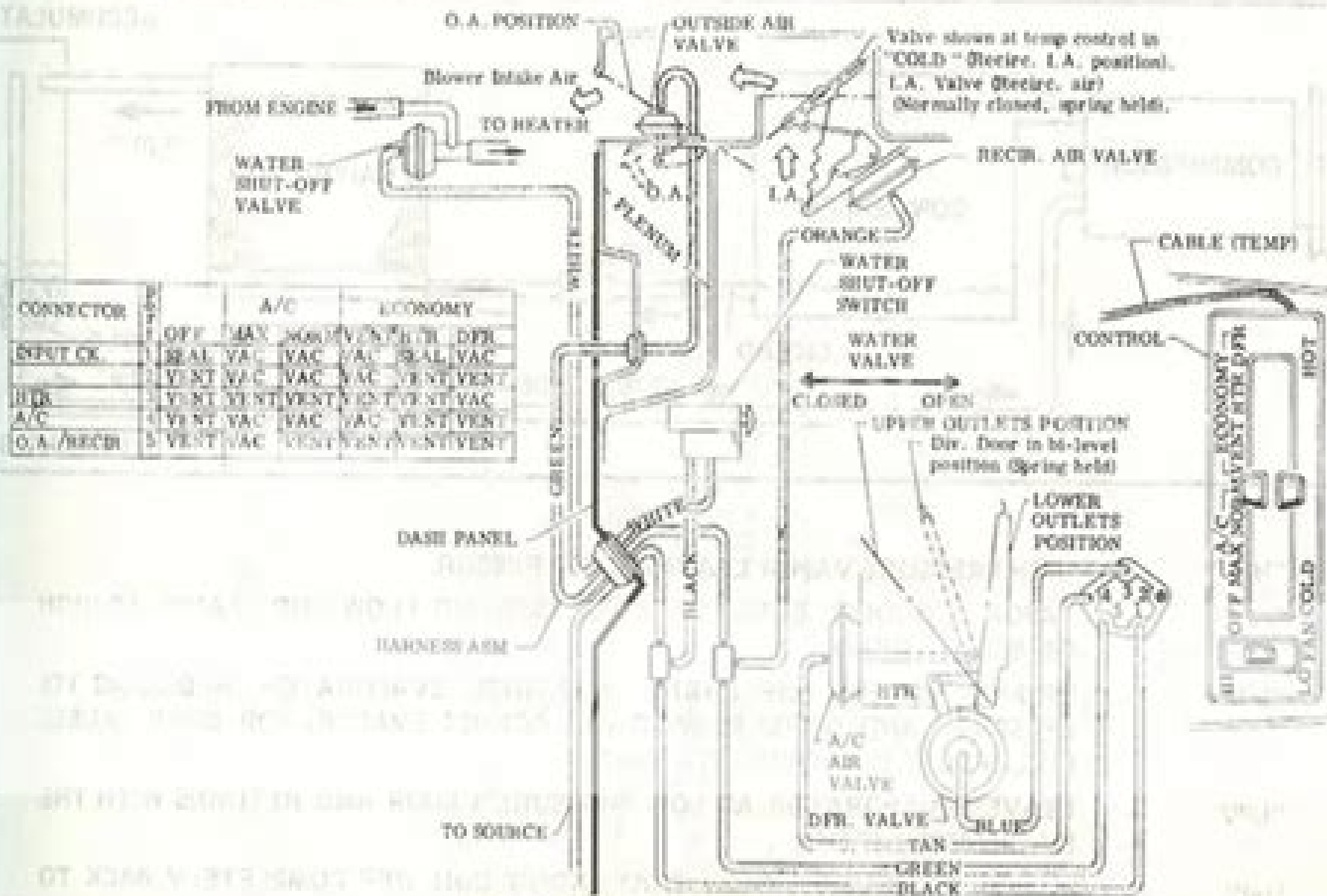
Fig. 1B-4-C60 A/C Vacuum Diagram
