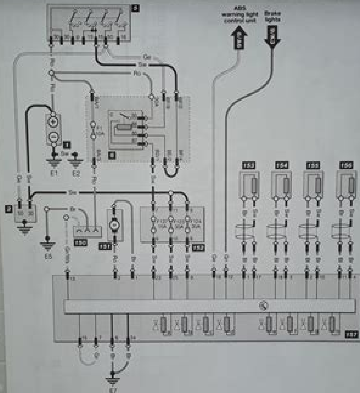
Diagram 12: Anti-lock braking system, models from March 1995
