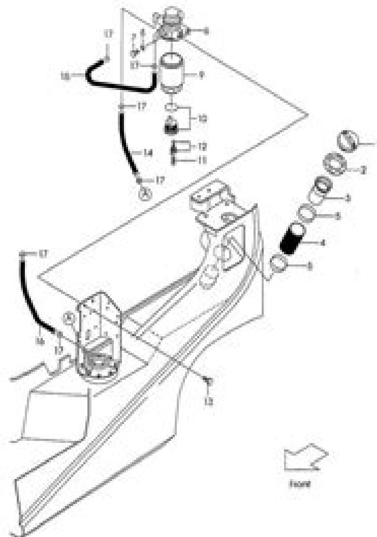
Fig.10 FUEL SYSTEM (D-TYPE) (P/F-PC200)
