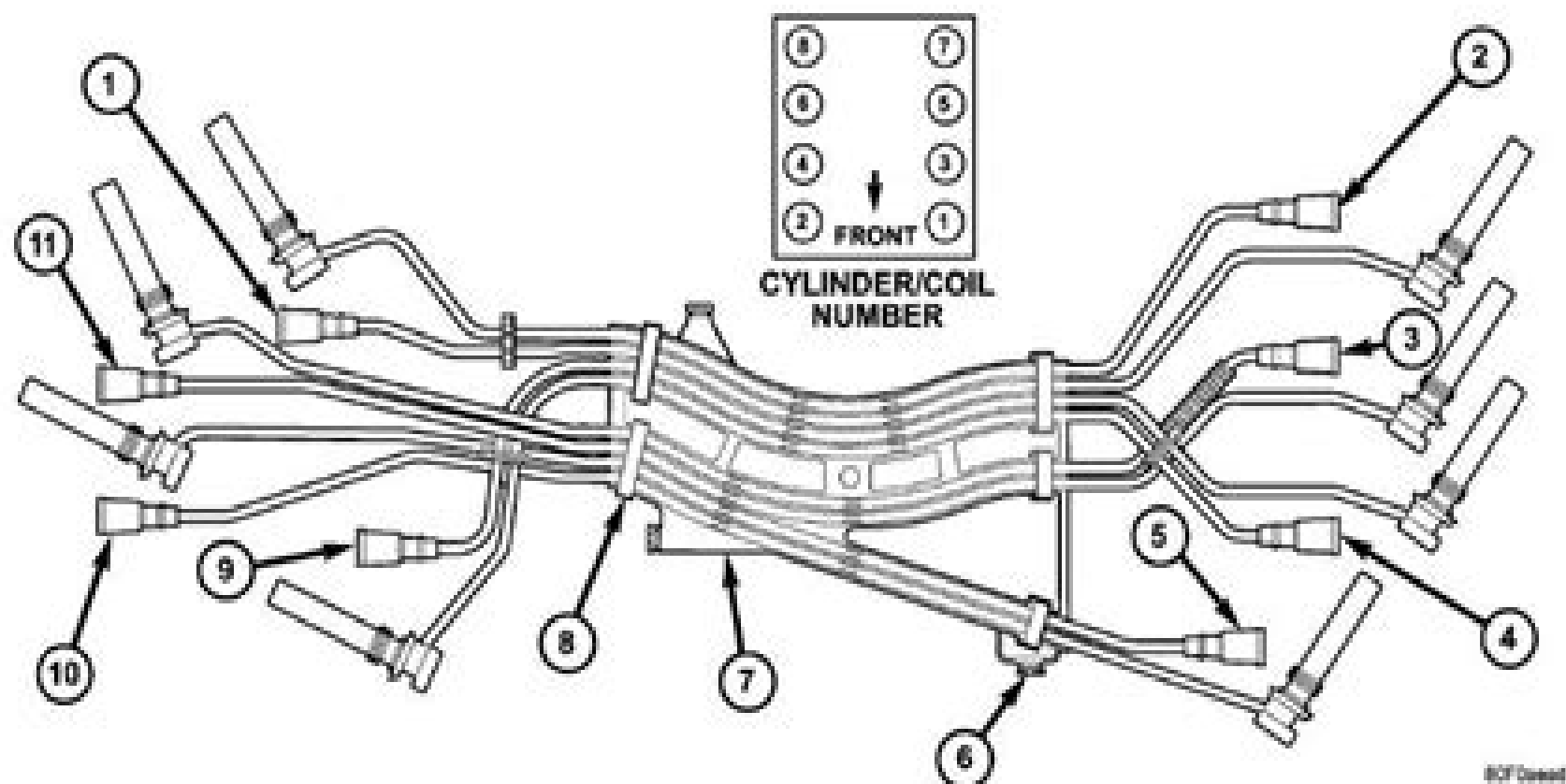
Fig. 22 5.7L SPARK PLUG CABLE ROUTING
