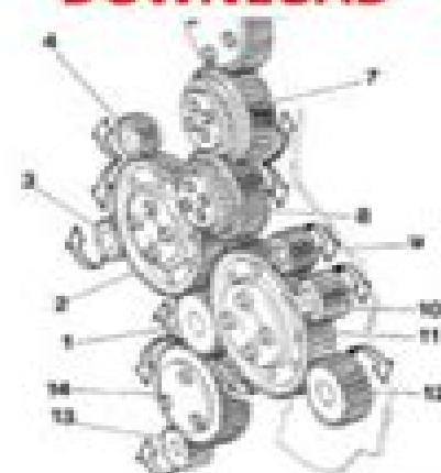
Fig. 1: Timing gear arrangement
