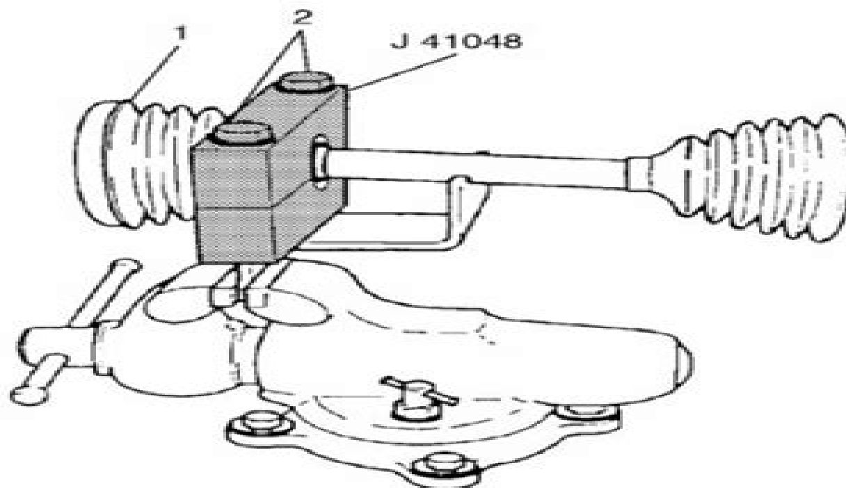
Fig. 43: Swaging Retaining Clamp Ring Courtesy of GENERAL MOTORS CORP.
