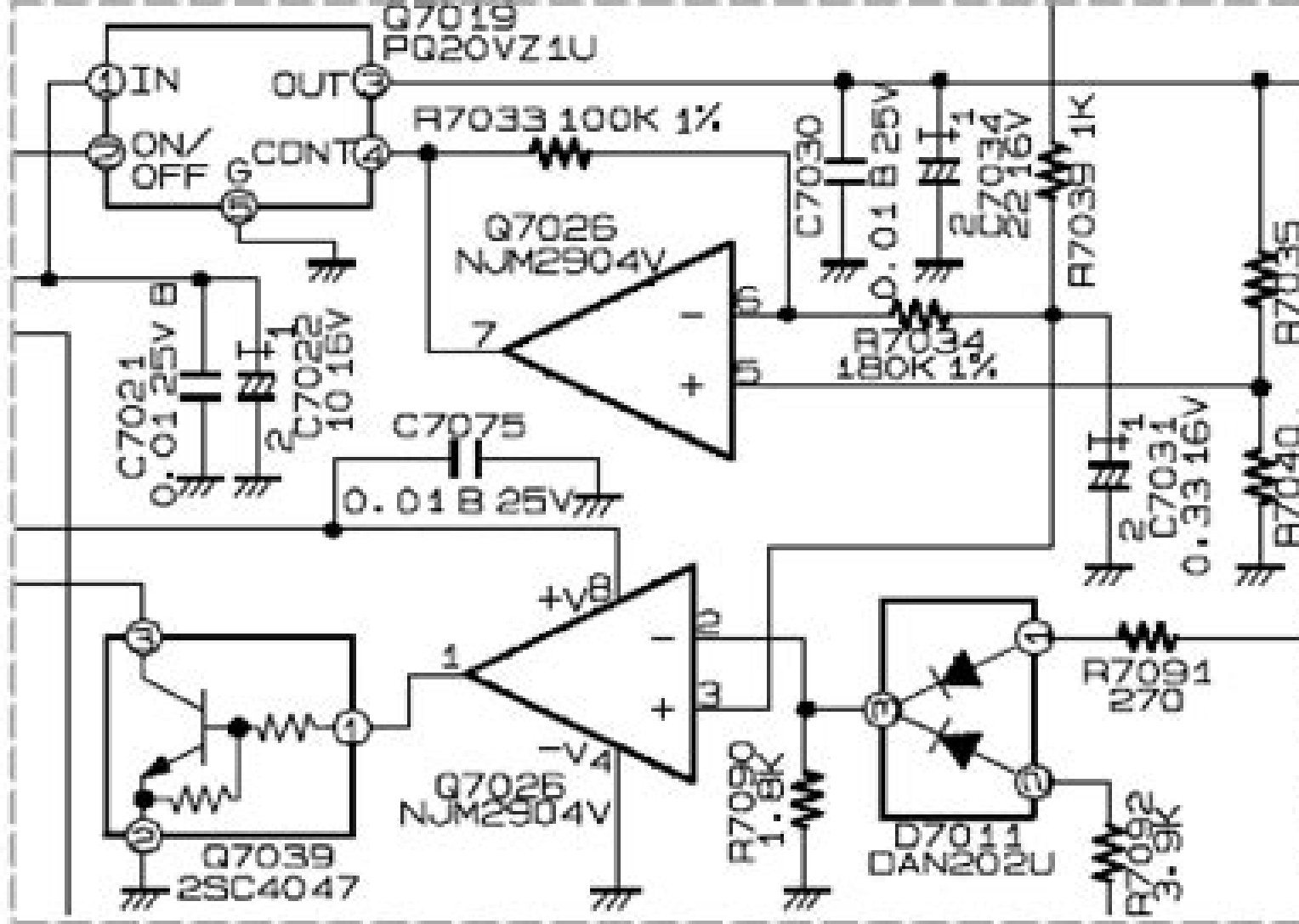
Preview: YAESU FT-100D schematic diagram
