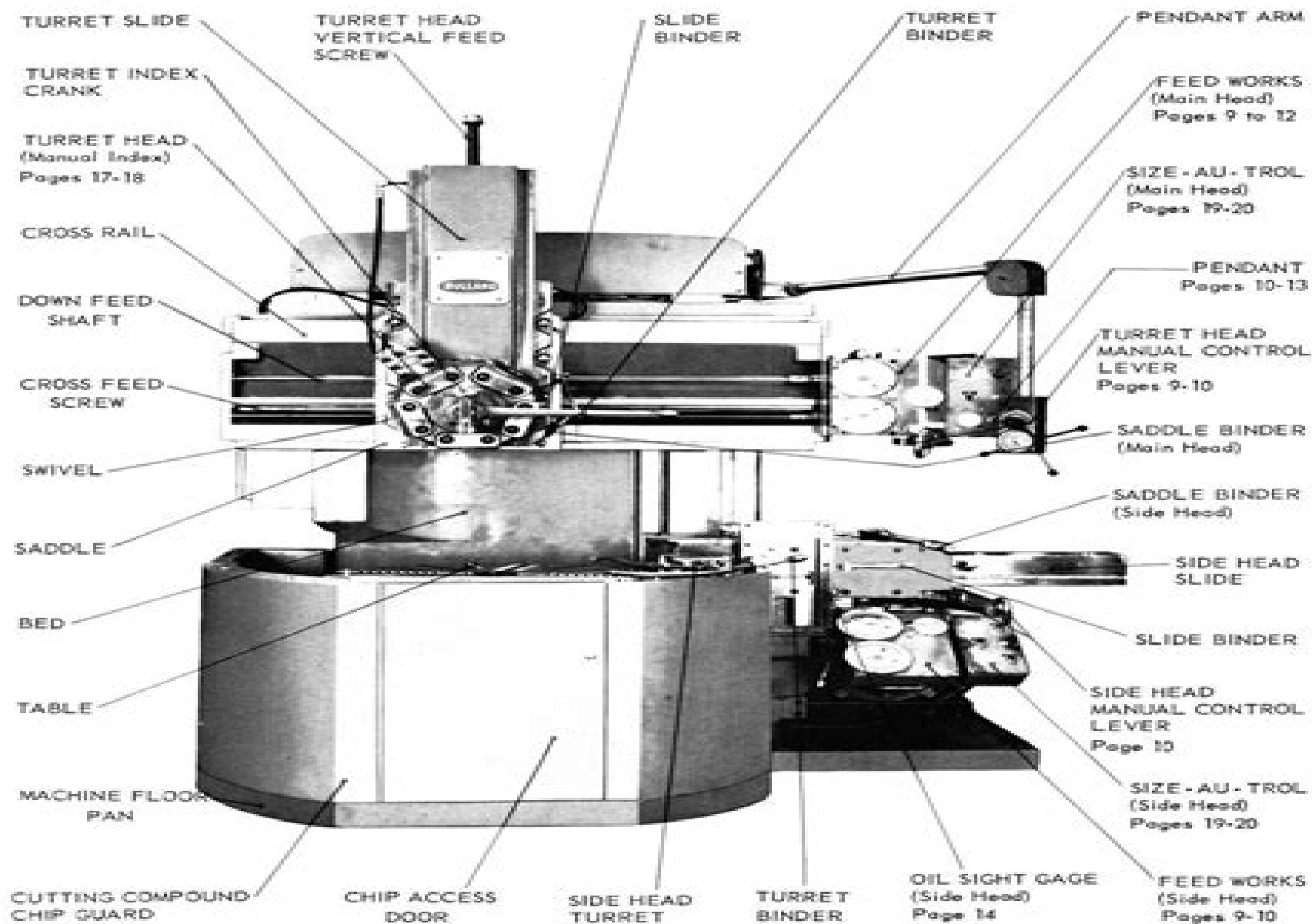
36" DYNATROL V. T. L. FRONT VIEW
