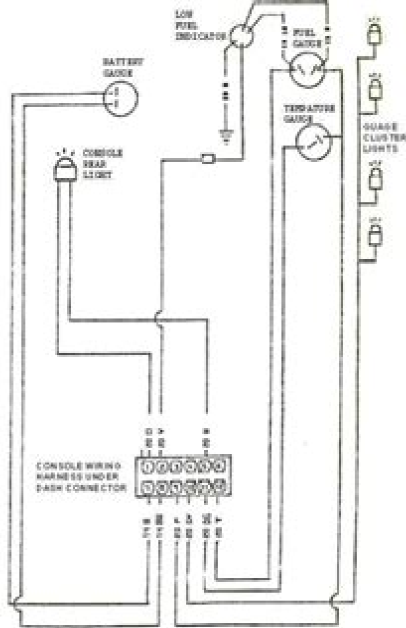
1948-1949 CONSOLE WIRING MANUAL TRANSMISSION WITH CONSOLE GAUGES
