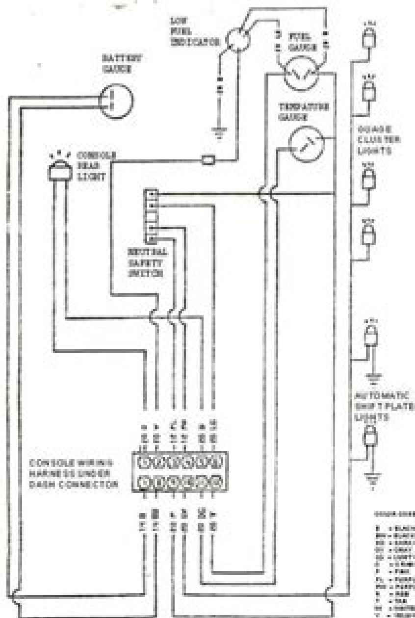
1948-1949 CONSOLE WIRING AUTOMATIC TRANSMISSION WITH CONSOLE GAUGES
