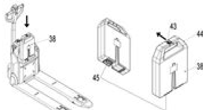
Fig. 35. Battery installation
