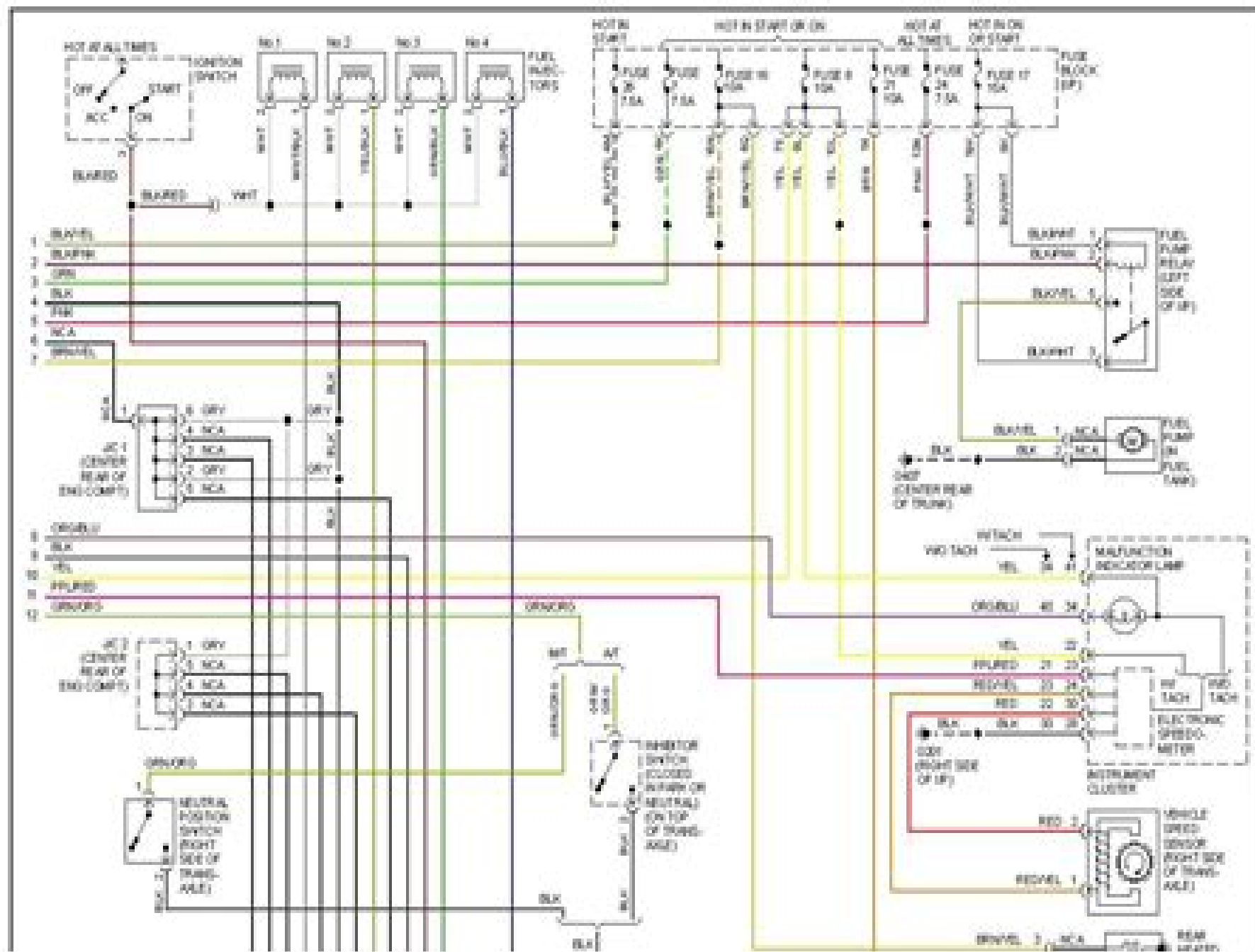
1995 Nissan Sentra GXE-Fig. 14: 1.6L, Engine Performance Circuits (2 of 2)
