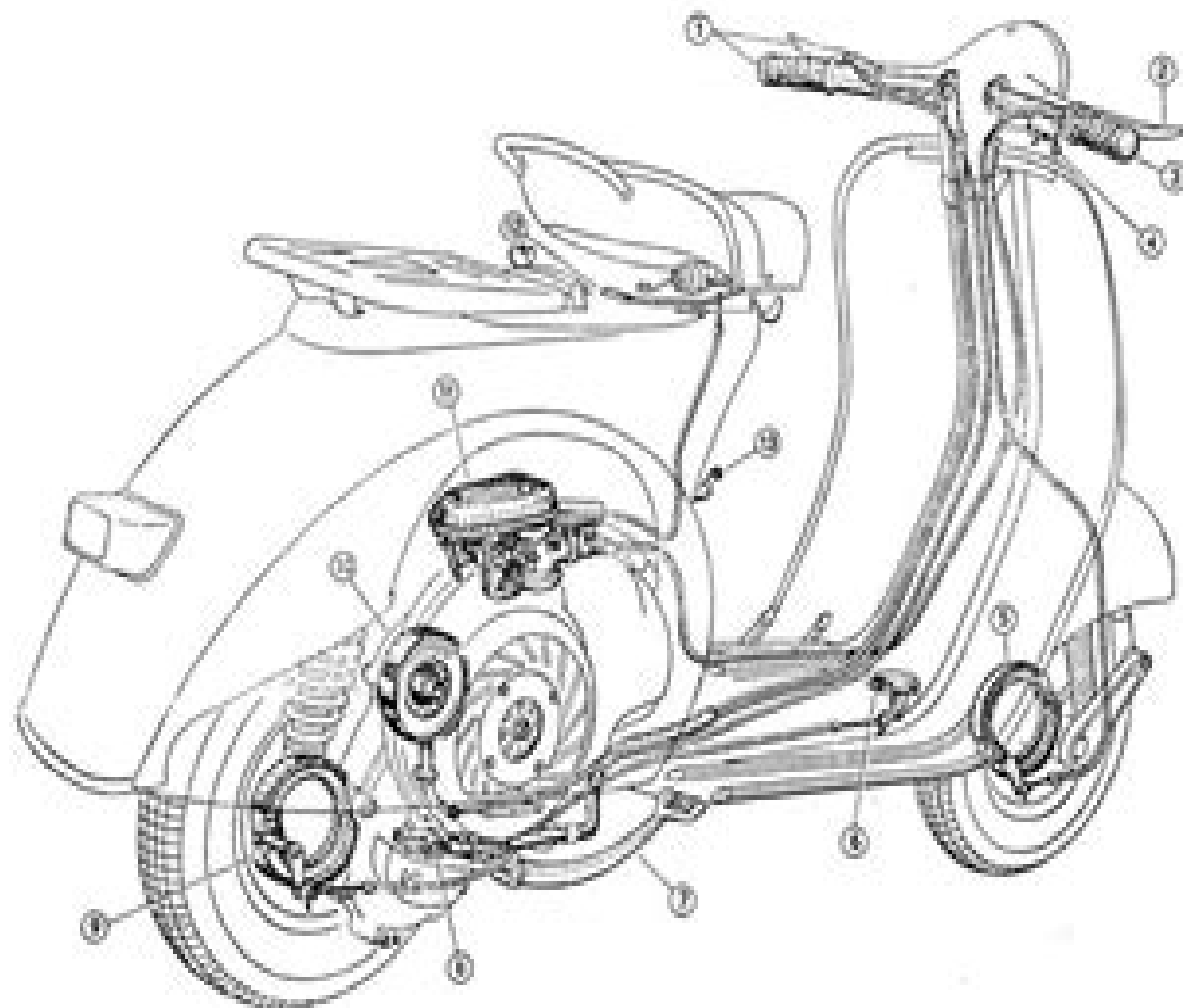
Fig. 3. Vespa controls.
