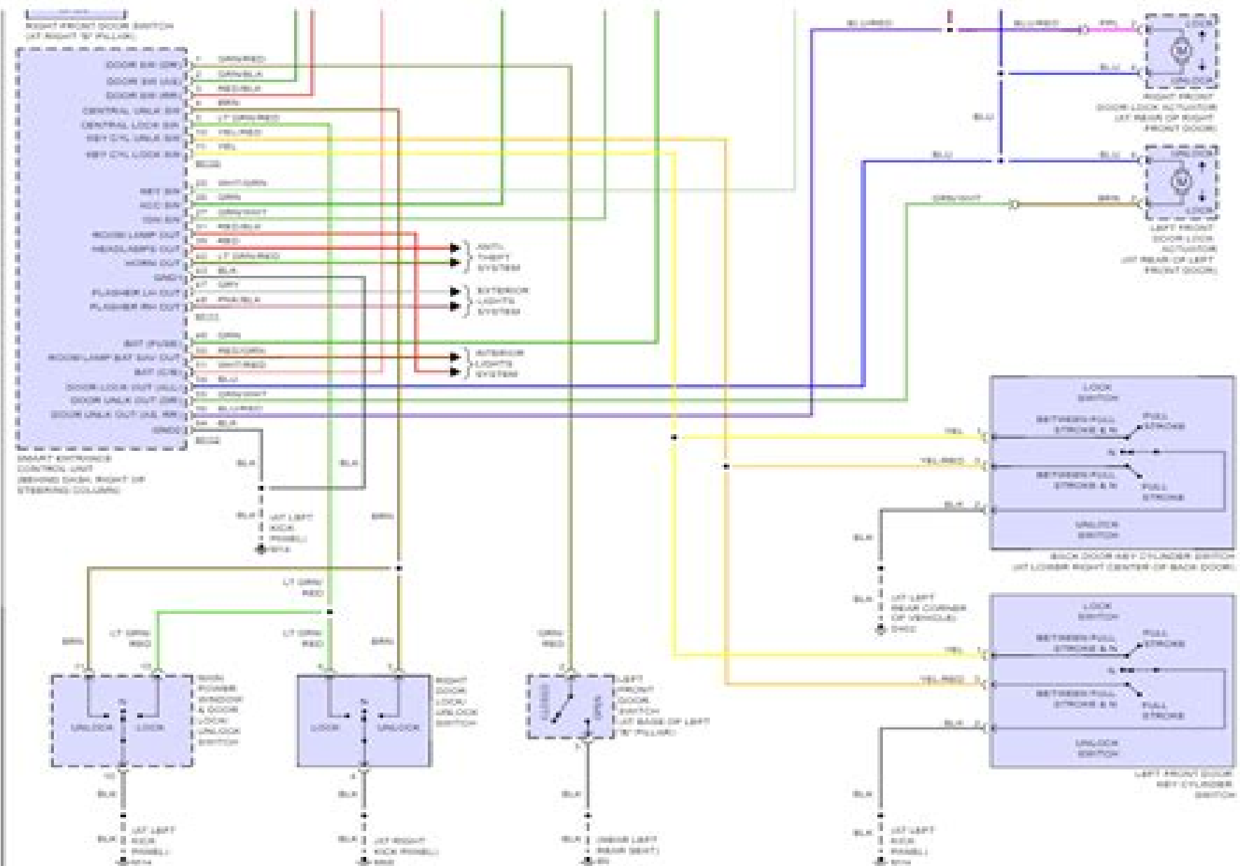
Fig 1: Power Door Locks Circuit
