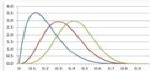
Beta Distribution
