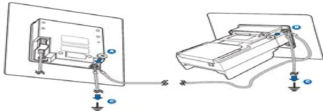
Figure 11 Grounding the UX300 and PIN Pad Units
