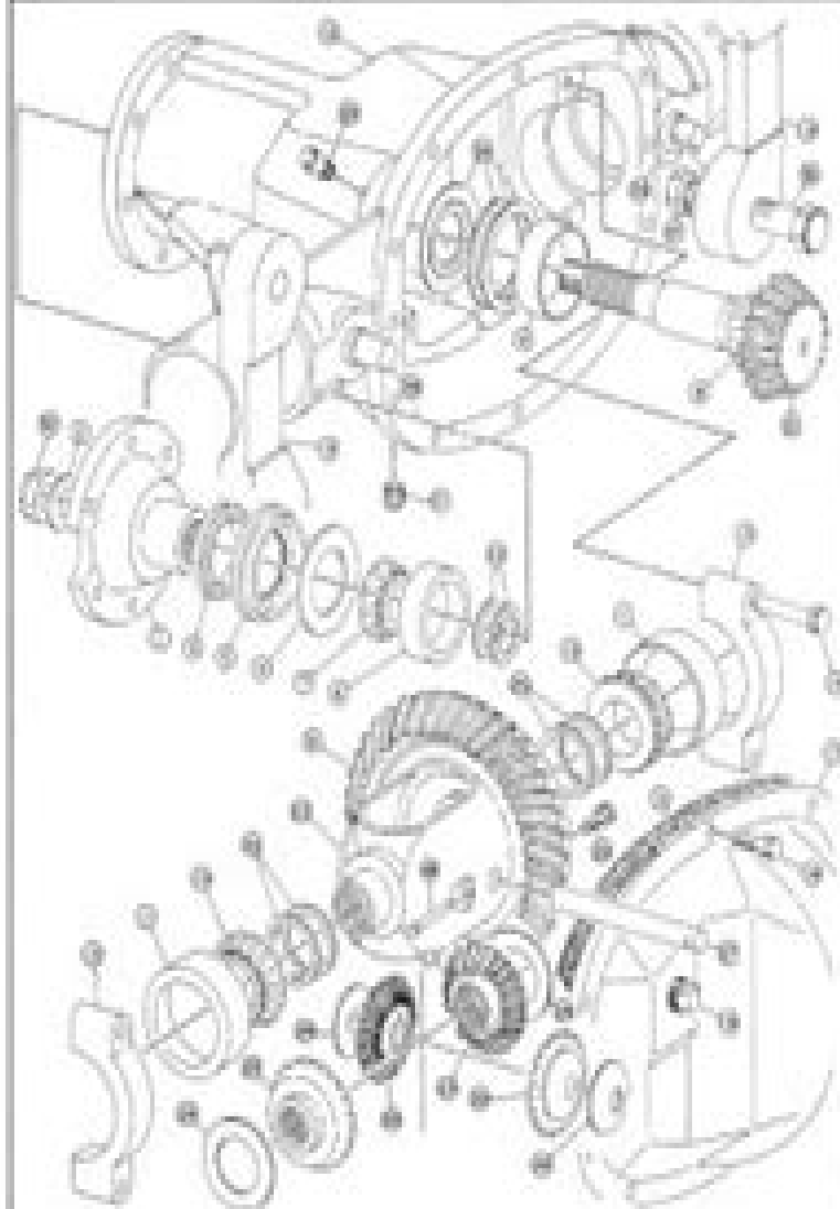
DRIVE AXLE CARRIER ASSEMBLY & INSTALLATION
