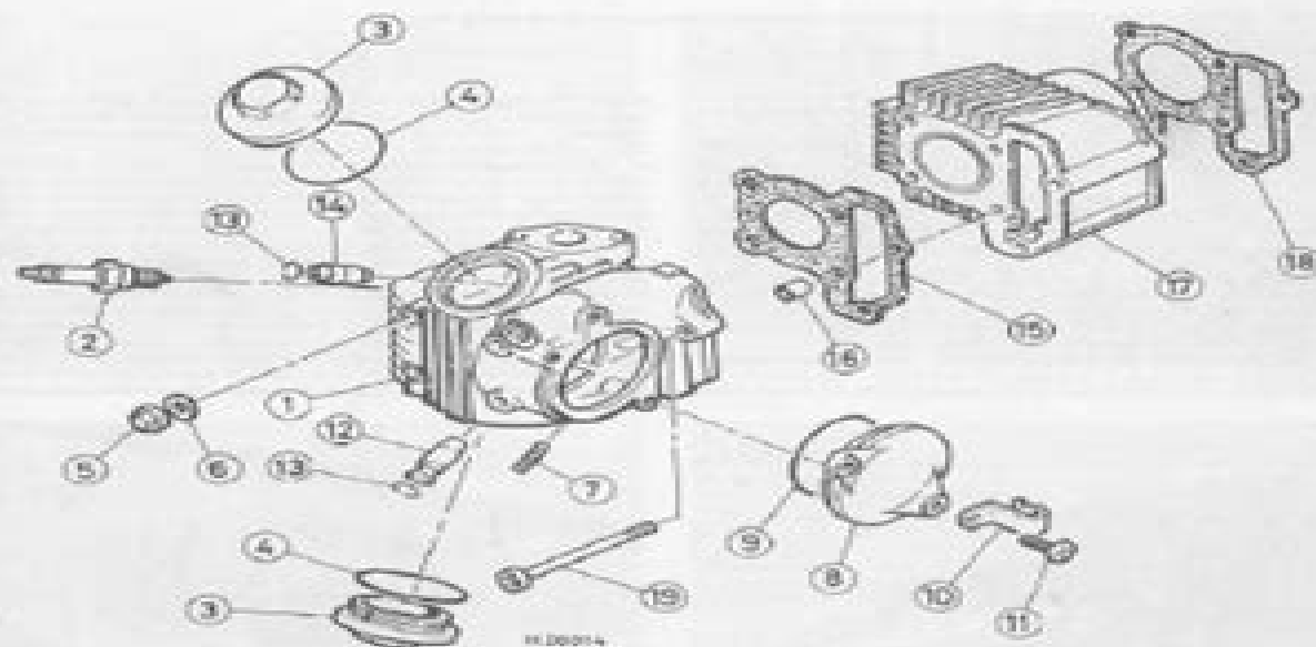
Fig. 1.1 Cylinder head and barrel
