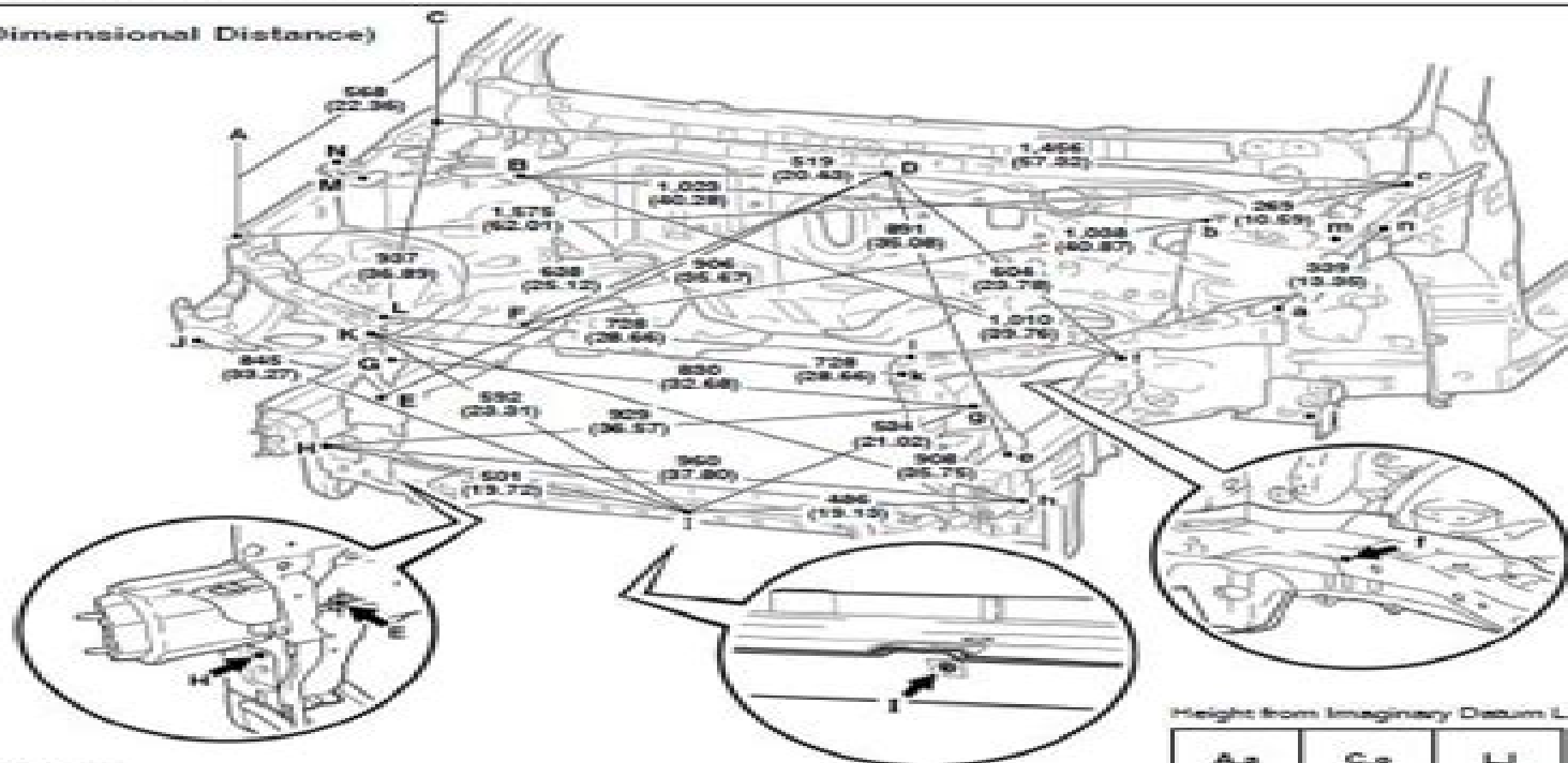
Vehicle Dimensions
