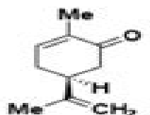
(S)-carvone
