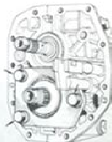
Fig. 6.27 Retorque the bearing endfloat plate onto the rear face of the 368 gearbox (See 6)
