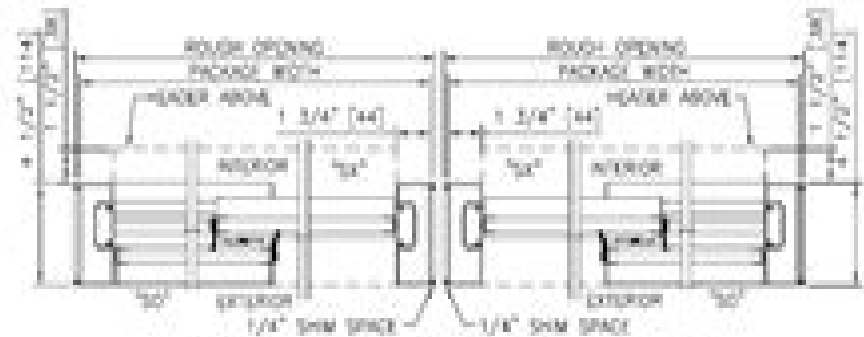
LEFT HAND HORIZONTAL SECTION RIGHT HAND SCALE 1" = 1'-0"
