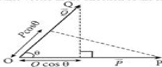
Fig. 2.9: Projection of vectors.
