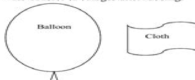
Balloon and cloth after rubbing
