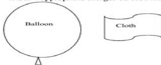
Balloon and cloth before rubbing
