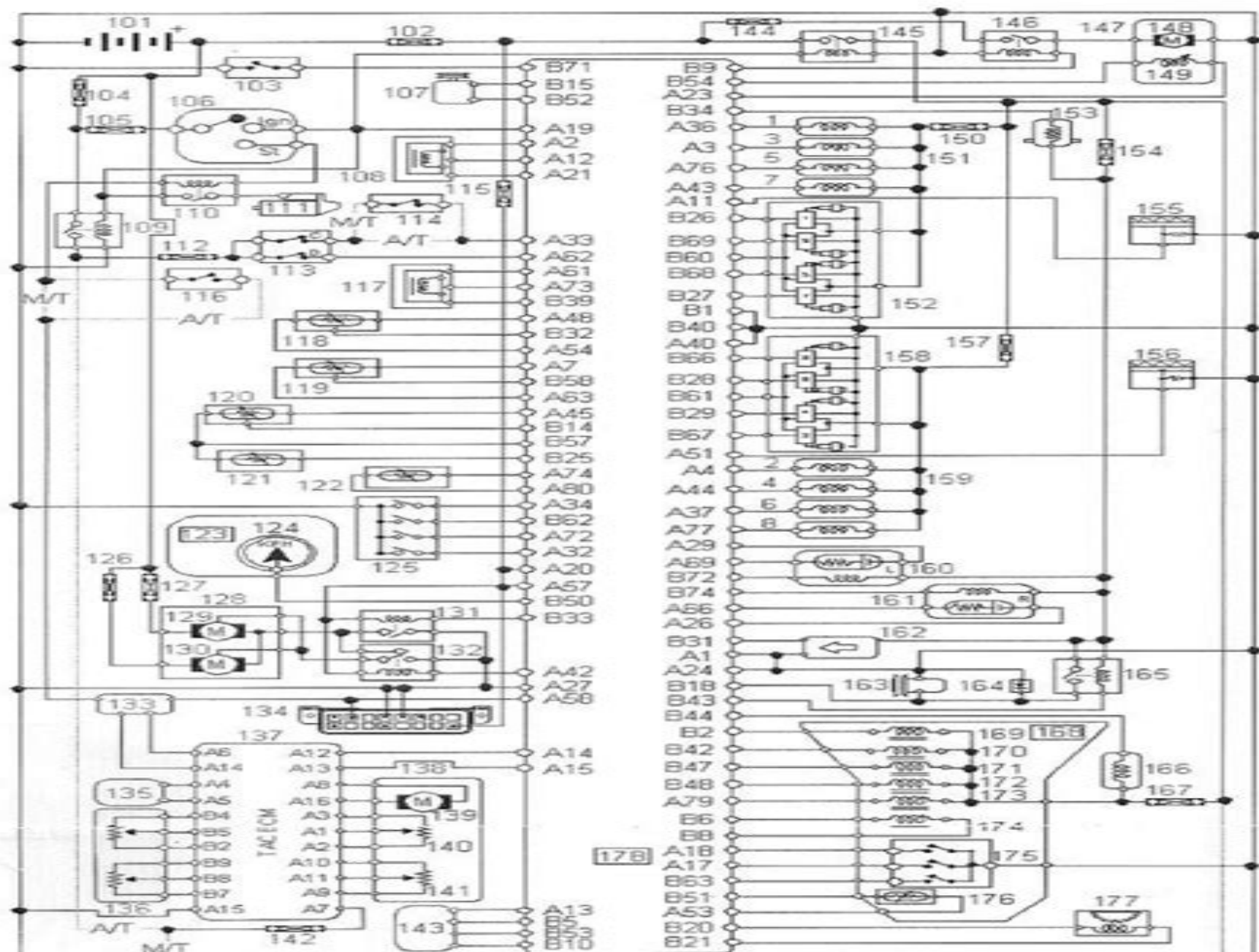
Holden 2004-06 5.7L V8 Engine and Transmission Wiring Diagram
