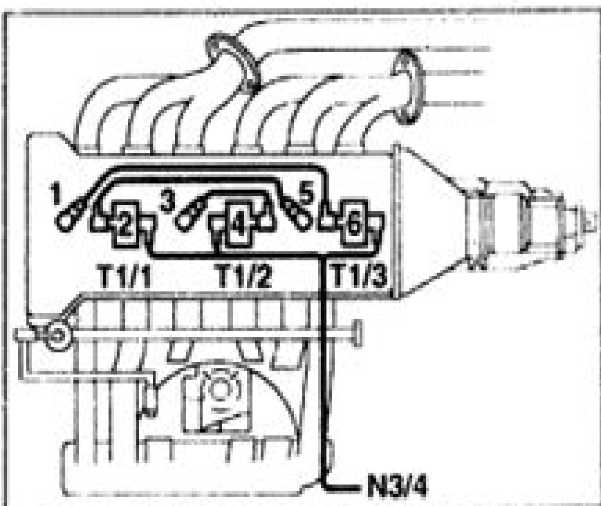
Left-hand illustration, engine 104 T1/1 Ignition coil cylinders 2 and 5 T1/2 Ignition coil cylinders 3 and 4 T1/3 Ignition coil cylinders 1 and 6 Firing order: 1-5-3-6-2-4
