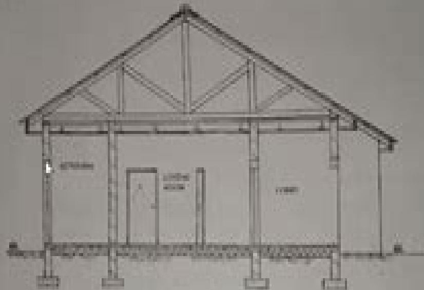
SECTION P-P
