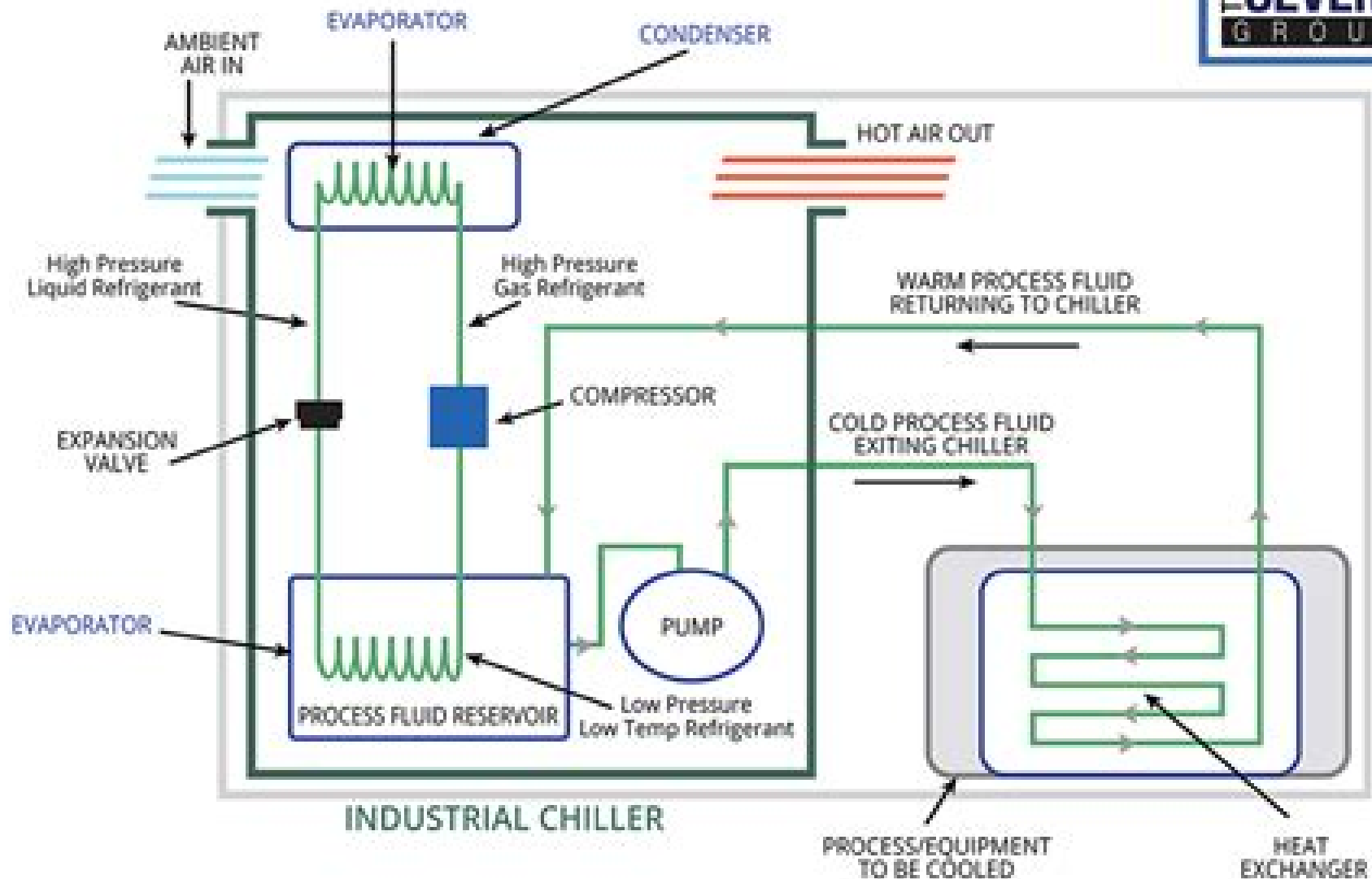
Figure 1 Schematic diagram of a typical chiller system
