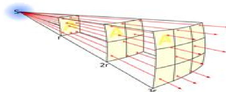
This picture depicts the inverse square law. When you move 2r away, the force is spread out over a space that is 4x as big and therefore the force is \frac{1}{4} as strong.
