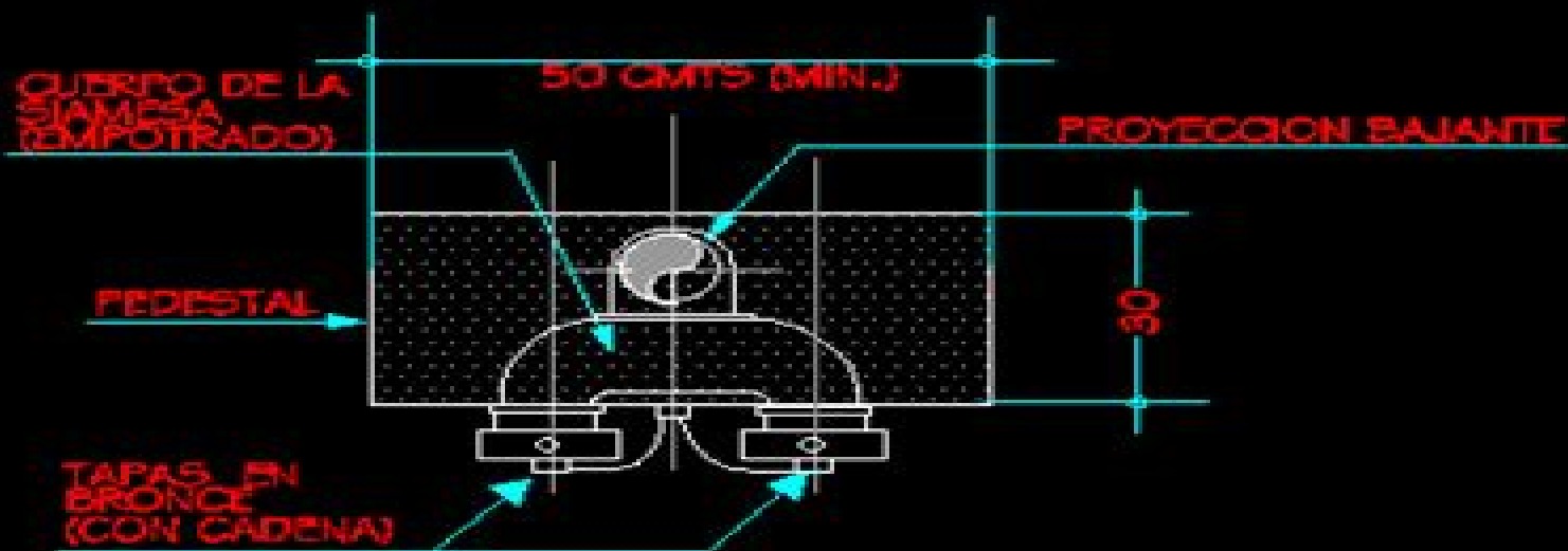
DETALLE PEDESTAL SIAMESA
