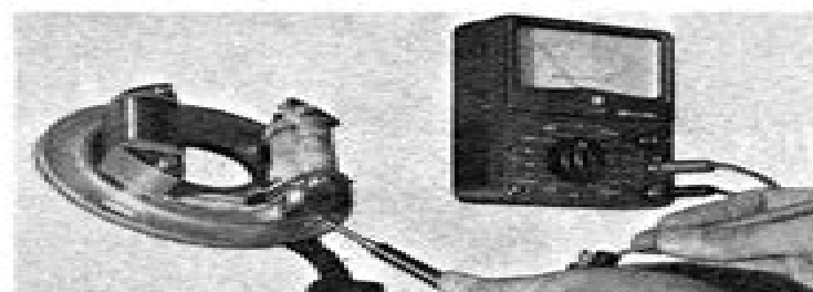
Fig. 8-5-1 Measure the resistance of exciter coil
