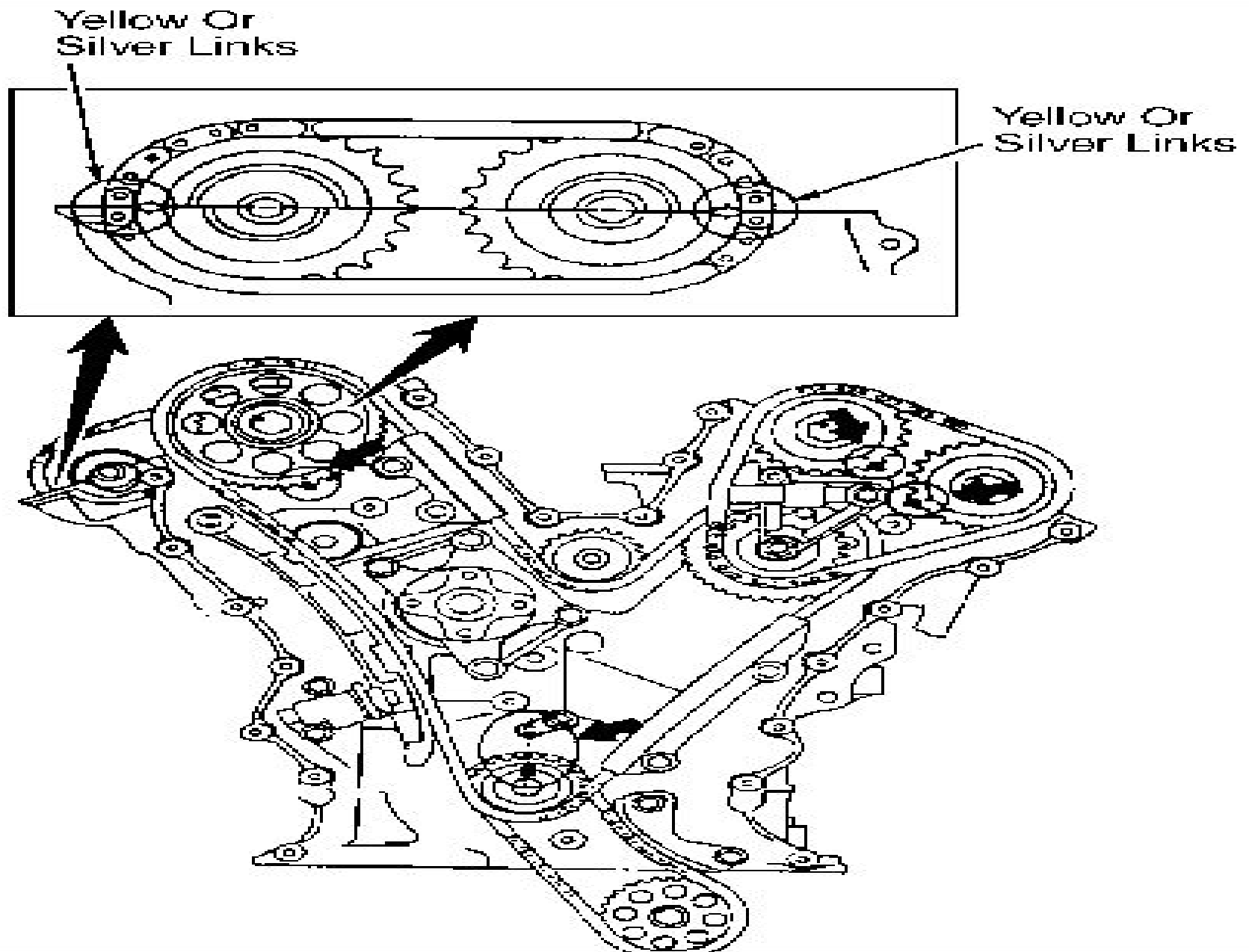
Fig. 14: Aligning Right Bank Timing Chain Courtesy of SUZUKI OF AMERICA CORP.
