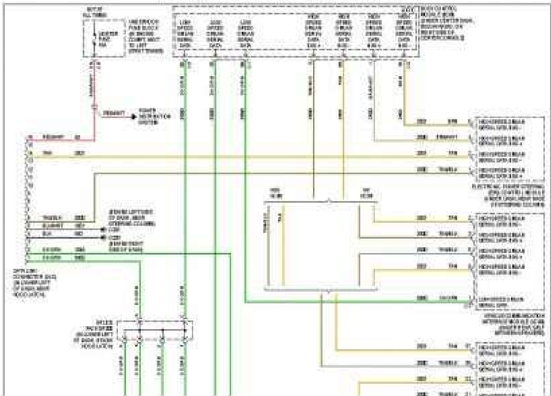
2006 Chevrolet Cobalt LS-Fig. 17: Computer Data Lines Circuit
