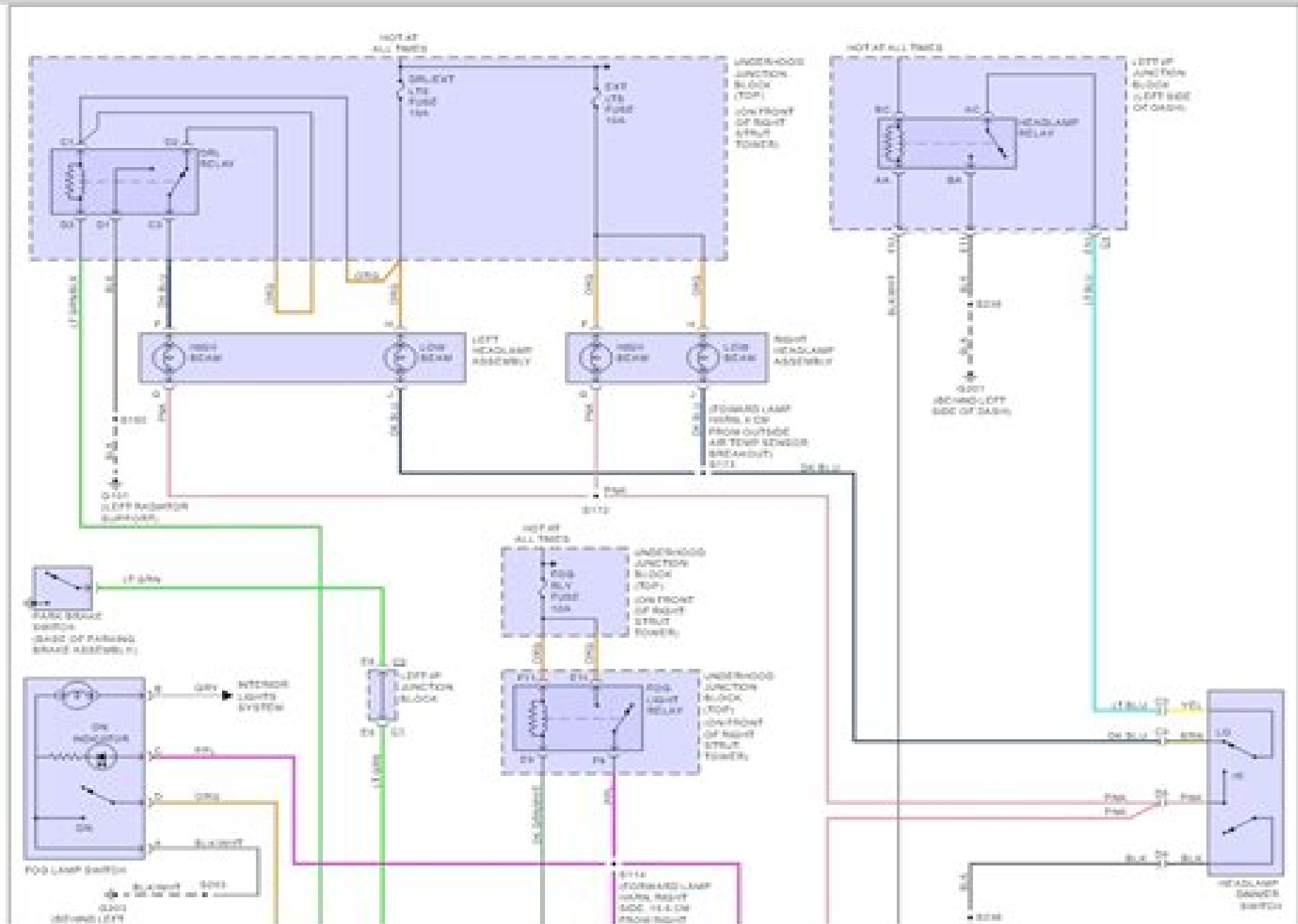
Fig 1: Headlights Circuit, W/O Police Or Emergency Vehicle Option
