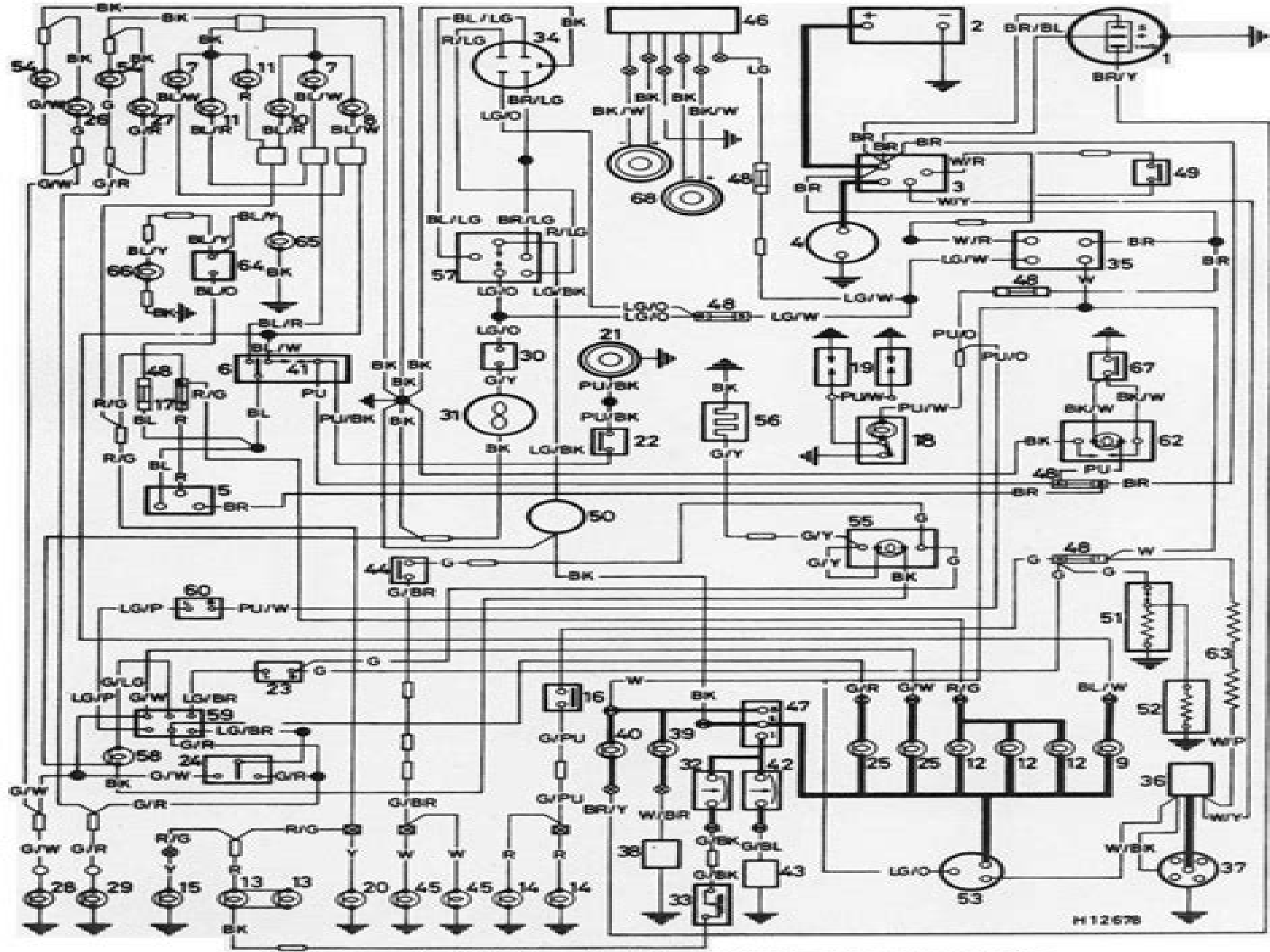
Wiring diagram 17 - all 1984-on carburettor models with multiple instrument pack
