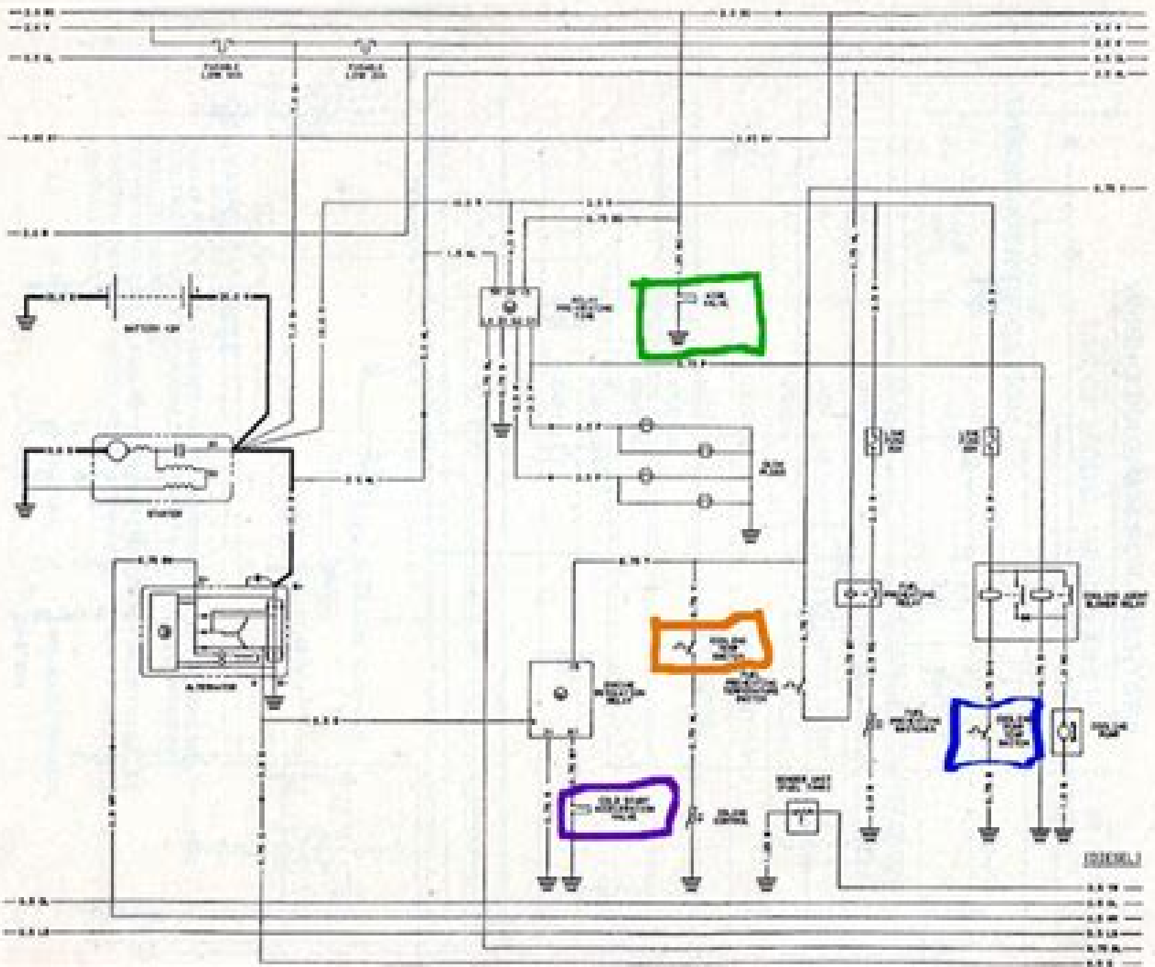
Typical wiring diagram (wiring provided) - continued
