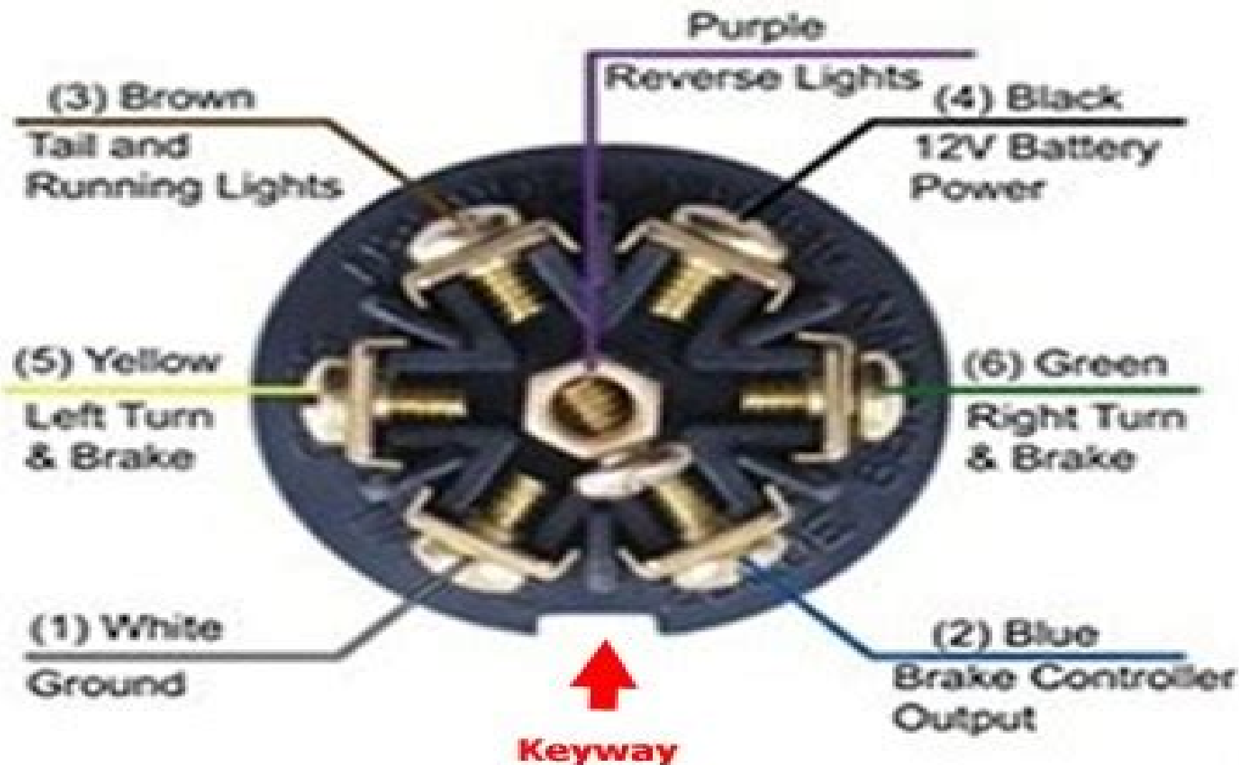
7-Way Blade Style Trailer Connector View from Back of Plug
