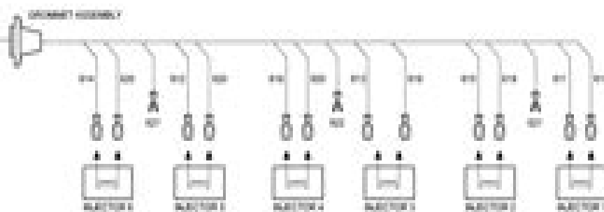
INJECTOR HARNESS SCHEMATIC (SERIES 60 WITH JAKE BRAKES SHOWN)
