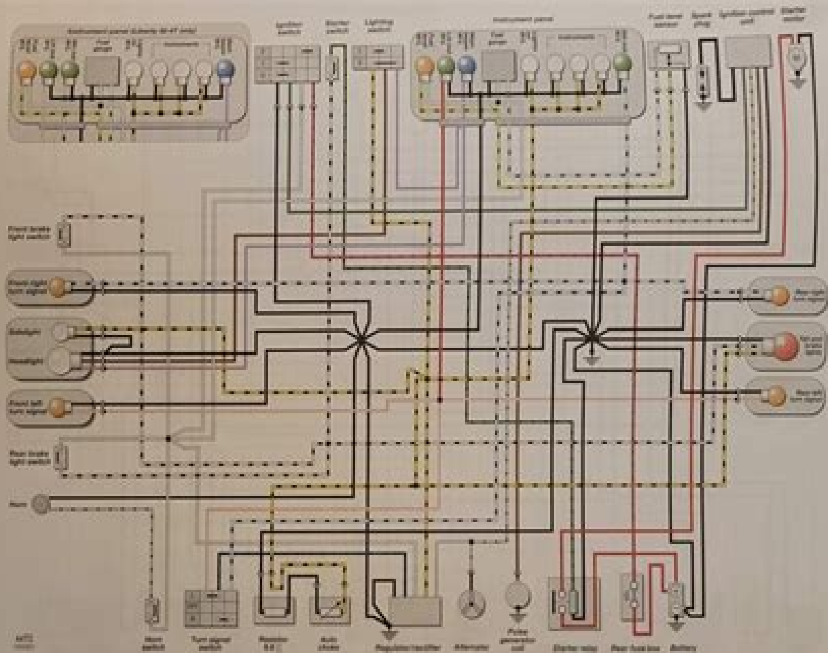
Zip 50-4T, Fly 50-4T, LX4 50 and Liberty 50-4T models
