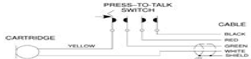
INTERNAL CONNECTIONS FIGURE 1
