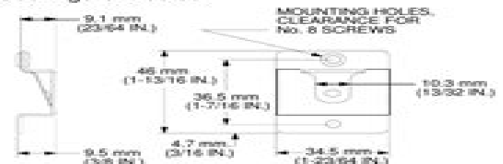
MOUNTING BRACKET FIGURE 2
