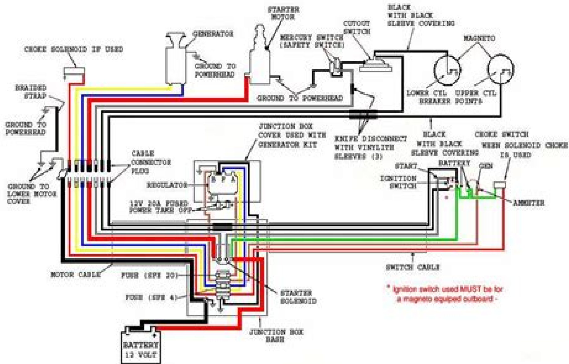
WIRING DIAGRAM FOR 1958-61 35 AND 40 HORSEPOWER MODELS (WITH GENERATOR KIT)
