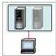
Enterprise Application
