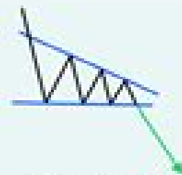
Descending Triangle
