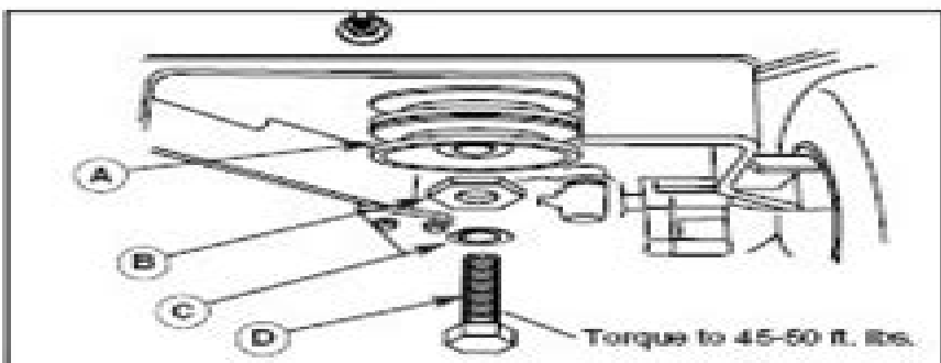
Figure 18. PTO (Electric Clutch) Assembly A. PTO Clutch B. Hex Washer C. Lockwasher D. Capscrew
