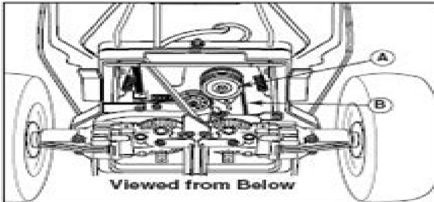
Figure 19. Disconnect Control Linkage A. Engine PTO Pulley B. Drive Belt
