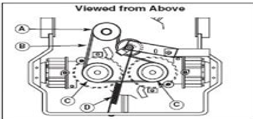
Figure 20. Transmission Drive Belt Routing A. Engine PTO Pulley B. Drive Belt C. Transmission Input Pulleys D. Belt Tension Spring
