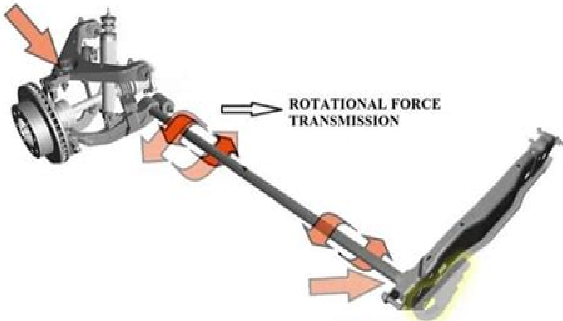
WORKING OF TORSION BAR
