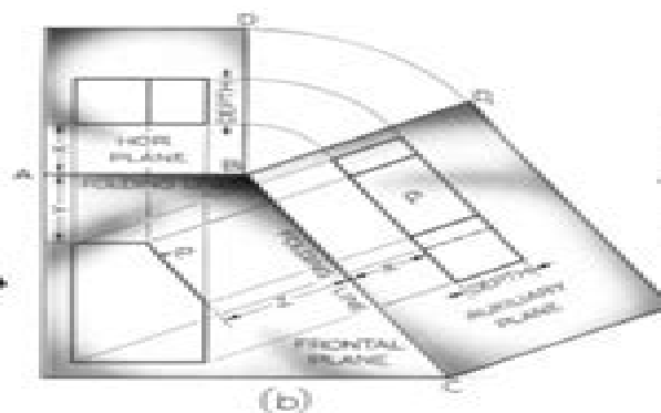
Figure 8-2 An Auxiliary View
