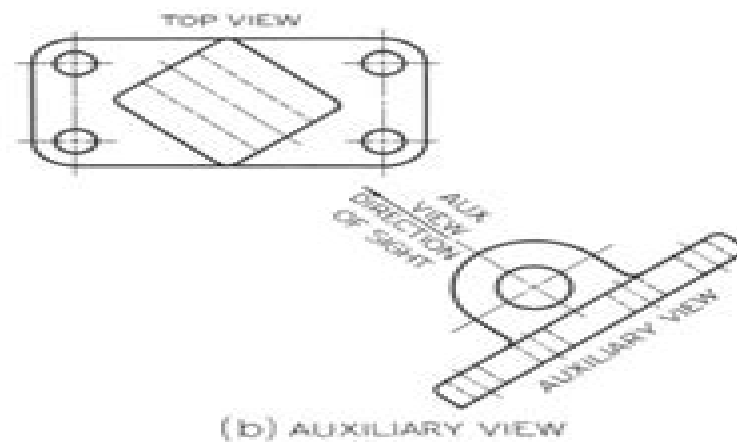
Figure 8-1 Regular Views and Auxiliary Views.
