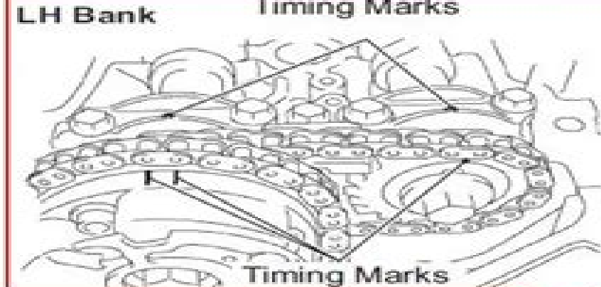
Timing Marks
