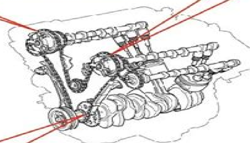
Timing Marks
